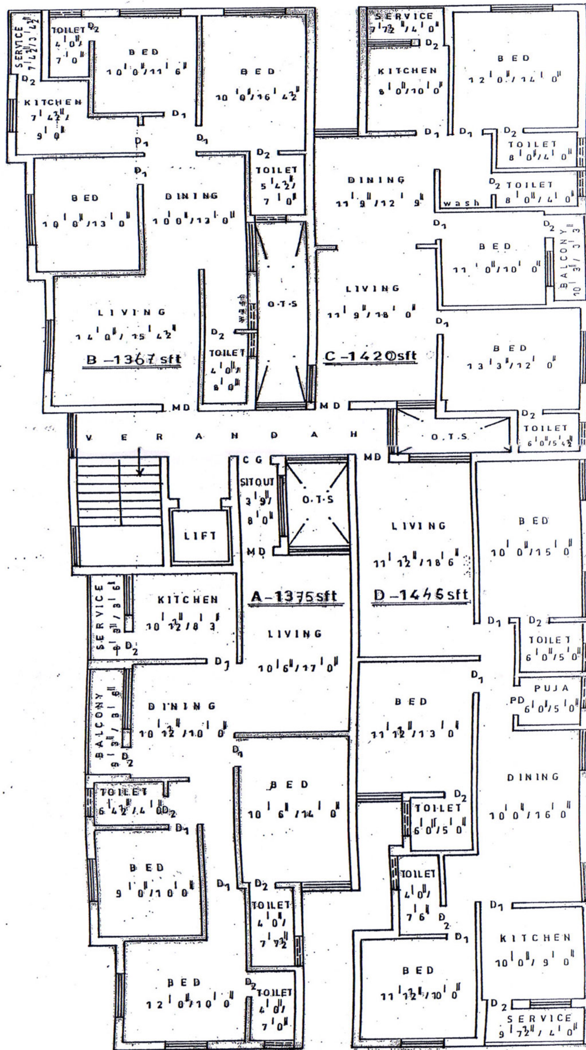
FIRST/SECOND FLOOR PLAN
